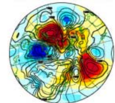
5-day Mean Sea Level Pressure 2000 1.15- 1.20 Contour Interval: 4hPa. Based Period for Normal 1981-90
