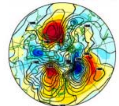
5-day Mean Sea Level Pressure 2000 1.21- 1.25 Contour Interval: 4hPa. Based Period for Normal 1981-90
