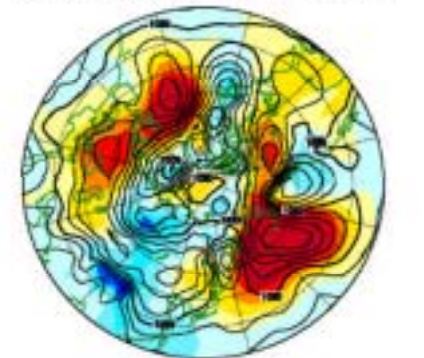
5-day Mean Sea Level Pressure 2000 1.11- 1.15 Contour Interval: 4hPa. Based Period for Normal 1981-90
