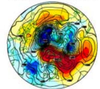
5-day Mean Sea Level Pressure 2000 1.5- 1.10 Contour Interval: 4hPa. Based Period for Normal 1981-90
